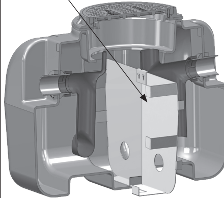
BIG-750-IB - with internal baffle
