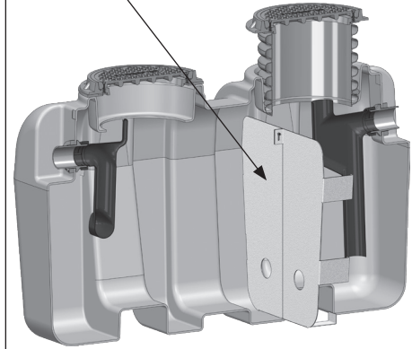
BIG-1150-IB - with internal baffle
