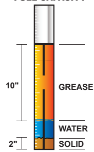
Lil-25 (25 GPM) CORE SAMPLE AT FULL CAPACITY
