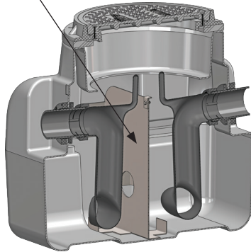
BIG-500-IB - with internal baffle
